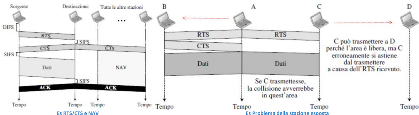
Es RTS/CTS e NAV
